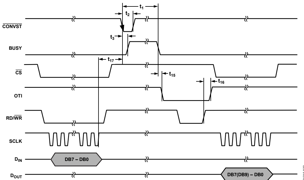
Figure 17. Mode 1 Operation
